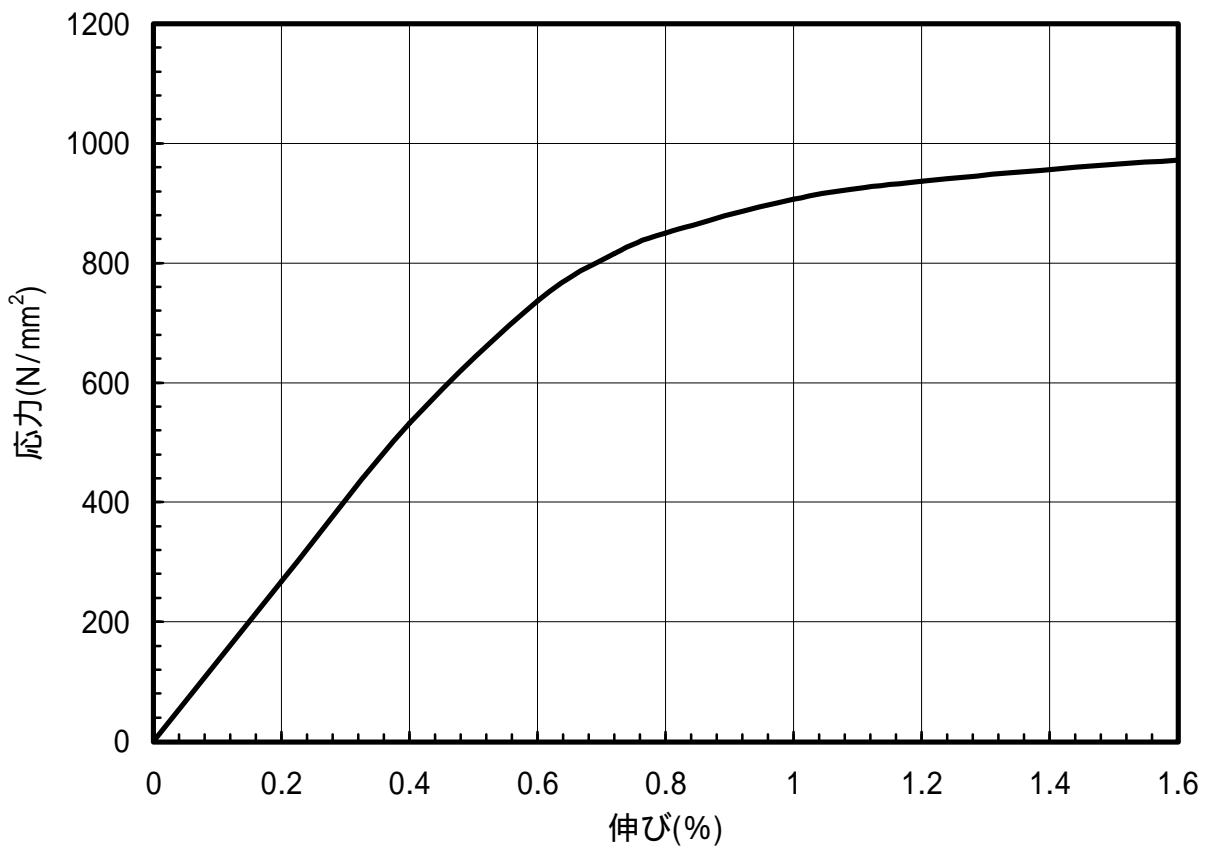
図 1.135 C1990-EHM材のS-S曲線(L.D.)
