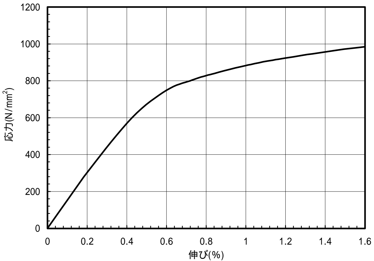
図 1.139 C1990-EHM材のS-S曲線(T.D.)
