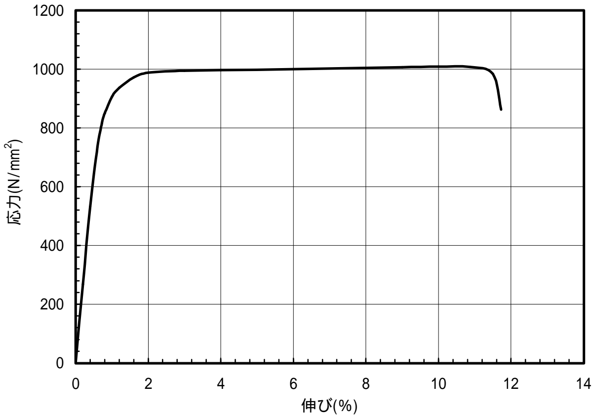
図 1.134 C1990-EHM材のS-S曲線(L.D.)
