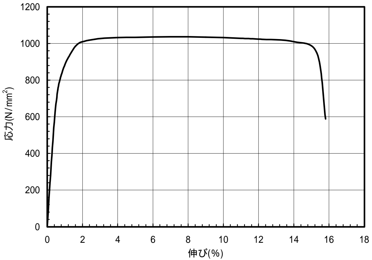
図 1.138 C1990-EHM材のS-S曲線(T.D.)
