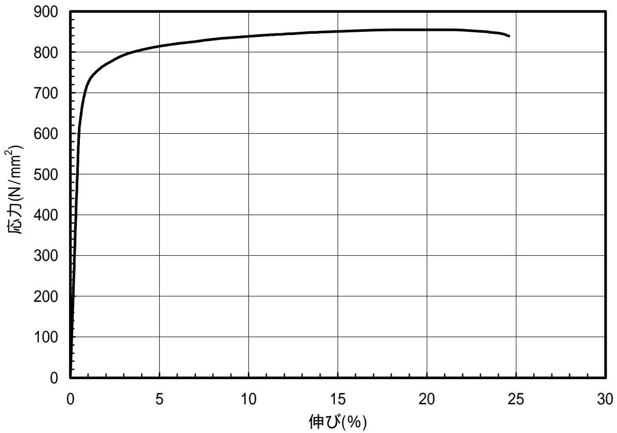
図 1.132 C1990-1/4HM材のS-S曲線(T.D.)
