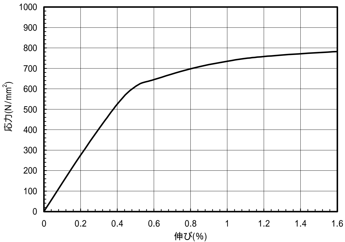
図 1.129 C1990-1/4HM材のS-S曲線(L.D.)
