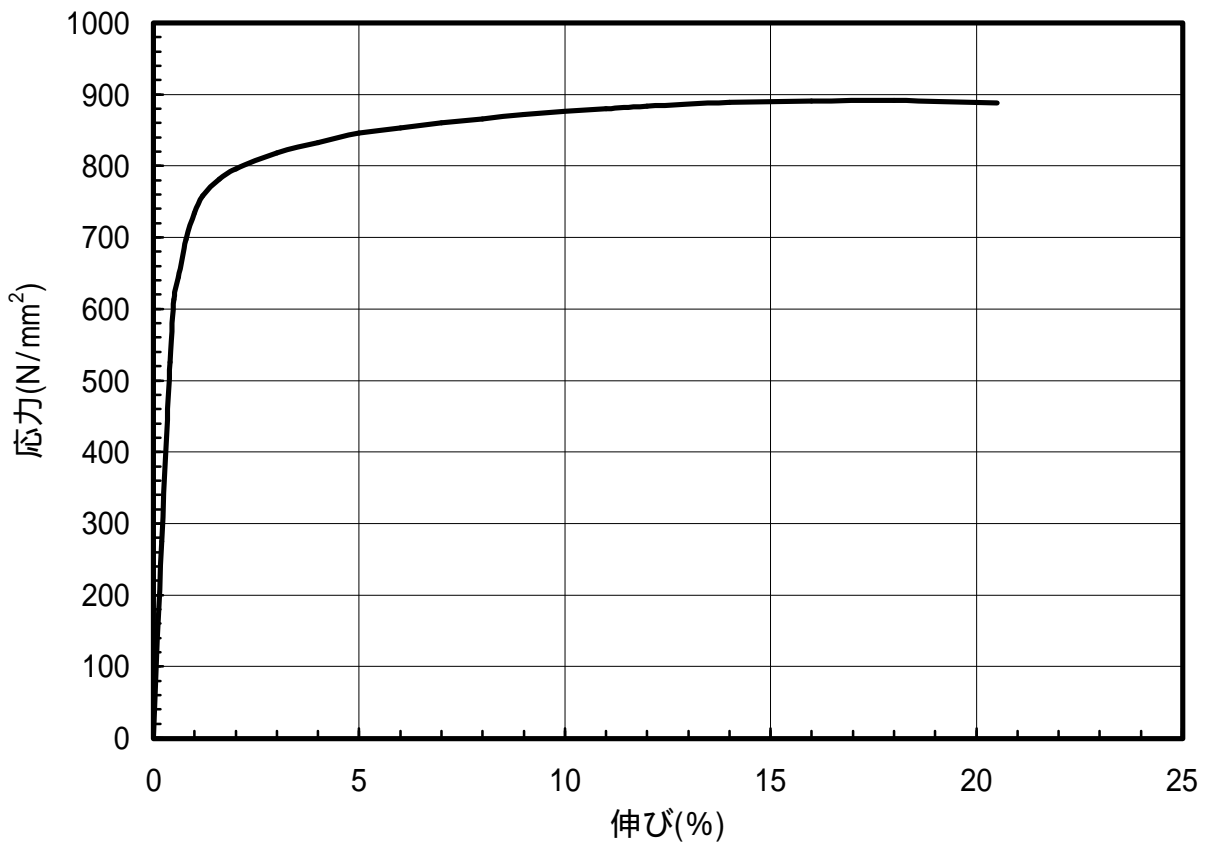
図 1.128 C1990-1/4HM材のS-S曲線(L.D.)
