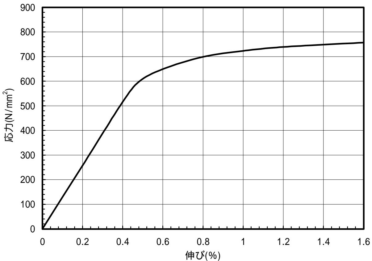
図 1.133 C1990-1/4HM材のS-S曲線(T.D.)
